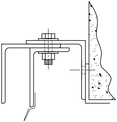
FACE OF WALL E-MOUNT TO STEEL
