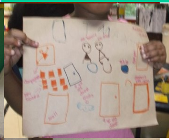
Class Map
