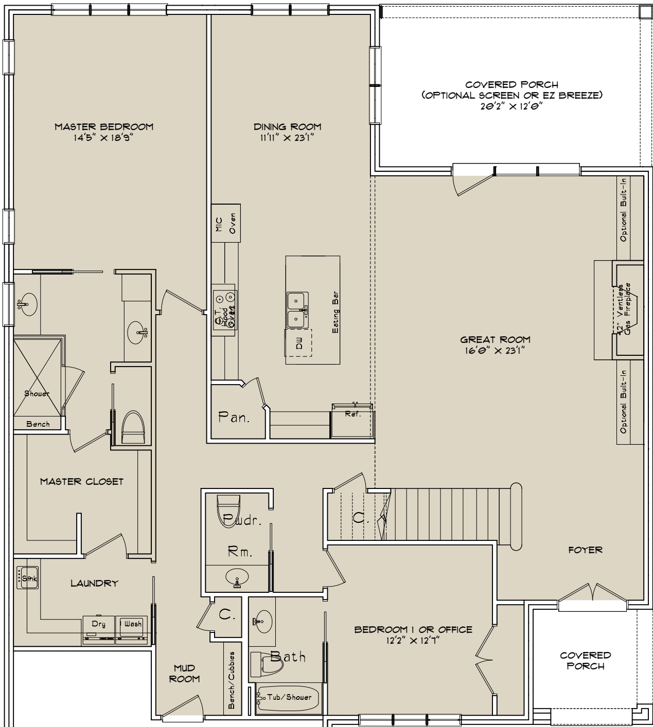
MAIN LEVEL PLAN
