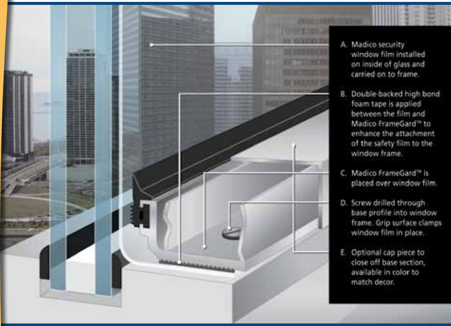
Madico FrameGard secures the film tightly in place to the window frame.
