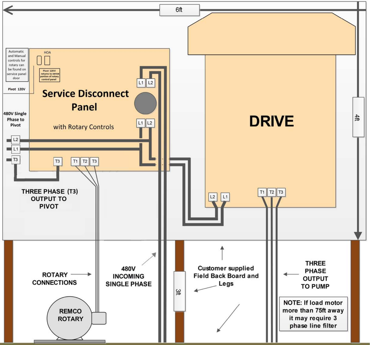
Recommended Cement Slab or Raised Platform for Rotary
