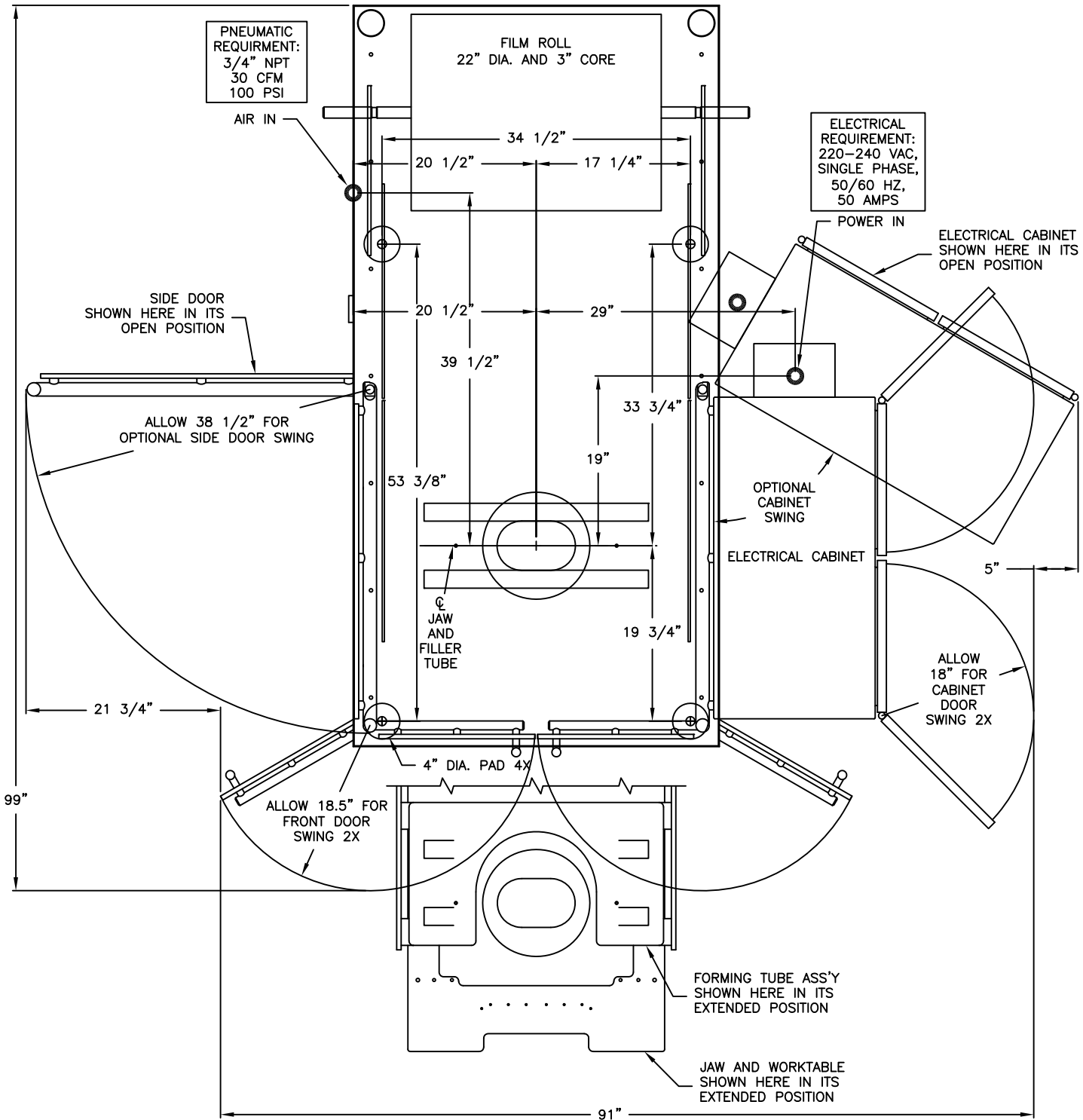
PACMAC MODEL 2016B FLOOR PLAN TOP VIEW
