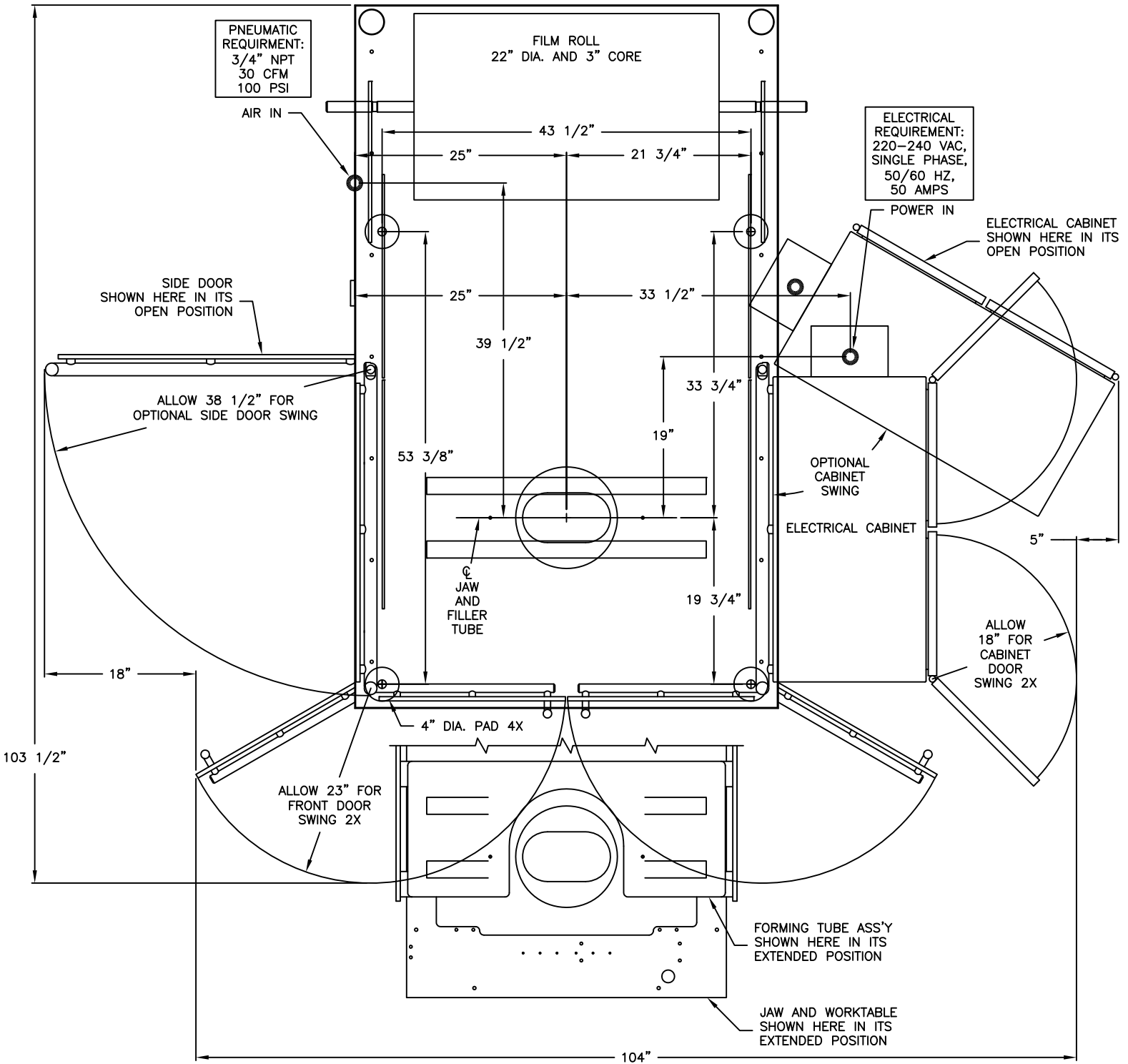
PACMAC MODEL 2015B FLOOR PLAN TOP VIEW
