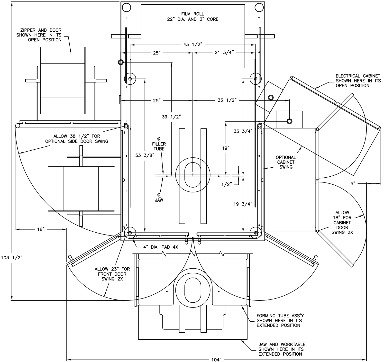
PACMAC MODEL 2015B3 FLOOR PLAN TOP VIEW
