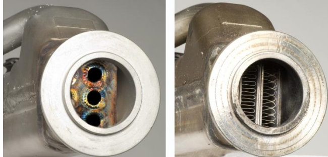
Above: Our upgraded EGR Cooler left, Ford Stock Part at Right
