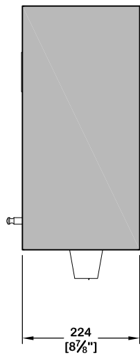
END VIEW
