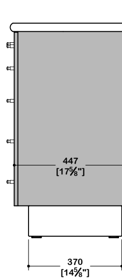
END VIEW
