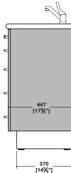
END VIEW
