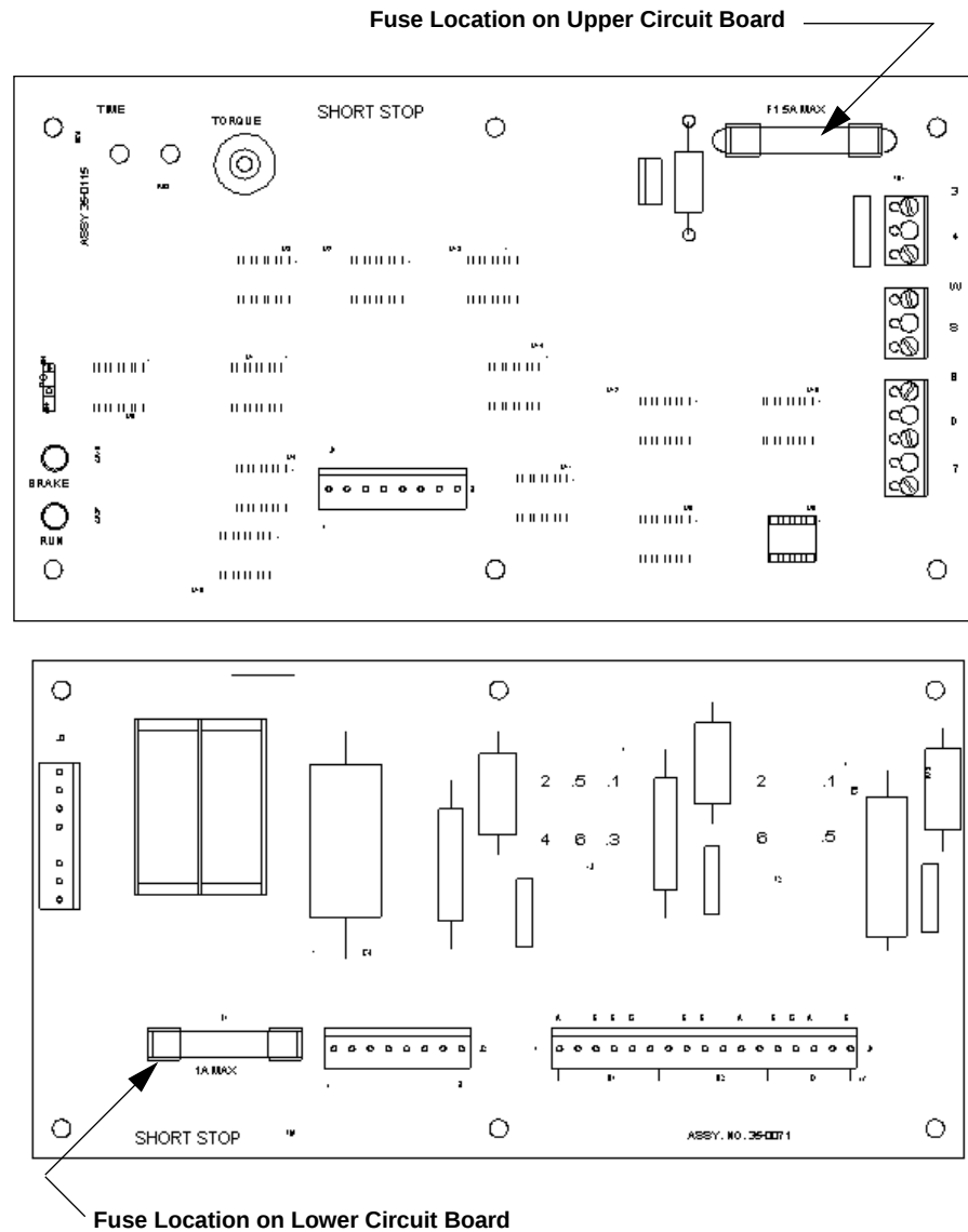
Figure 12: Location of PCB Fuses
