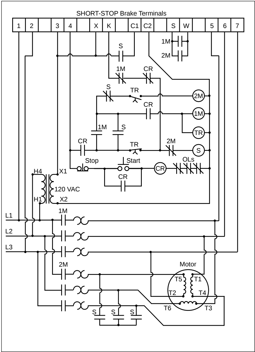
Figure 8: Power Connections in an Application with a Wye-Delta Starter
